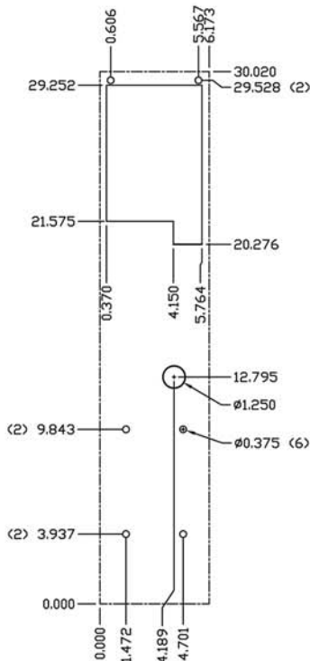
CUTOUT DRAWING
