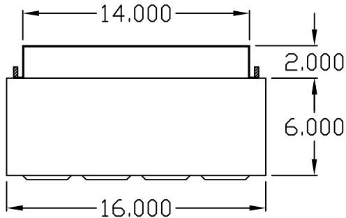
IQ3600HEV TOP VIEW
