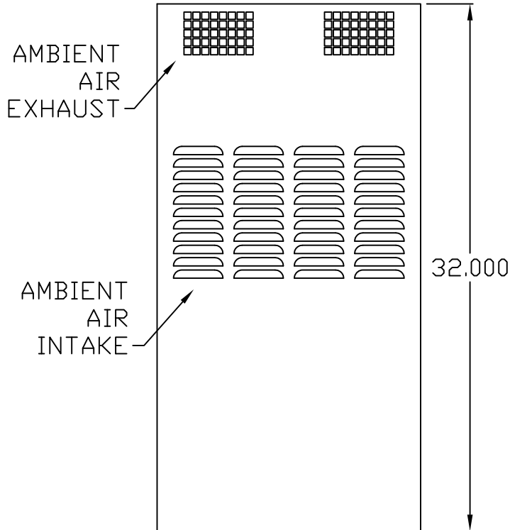
IQ3600HEV FRONT VIEW
