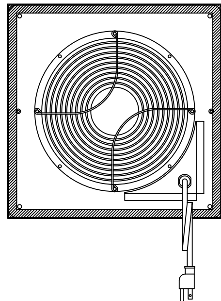
IQ500FP GASKET DRAWING
