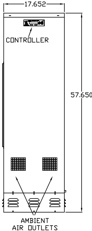
IQ8000VHA IQ10000V IQ12000V FRONT VIEW
