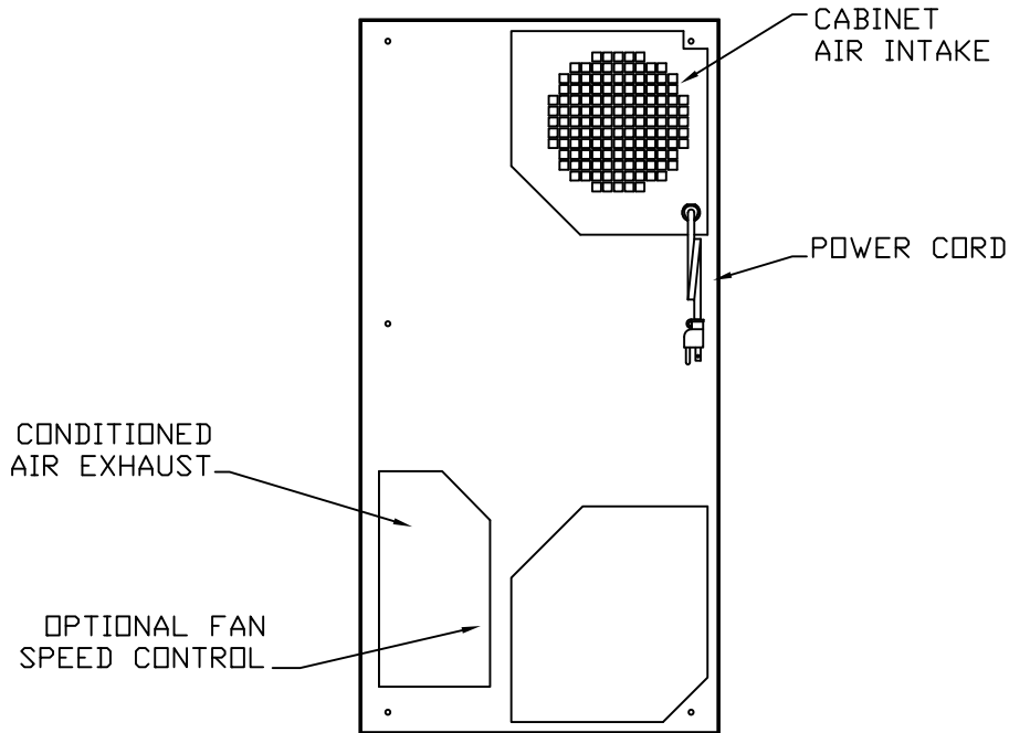
IQ7400HE-XF CUT OUT DRAWING
