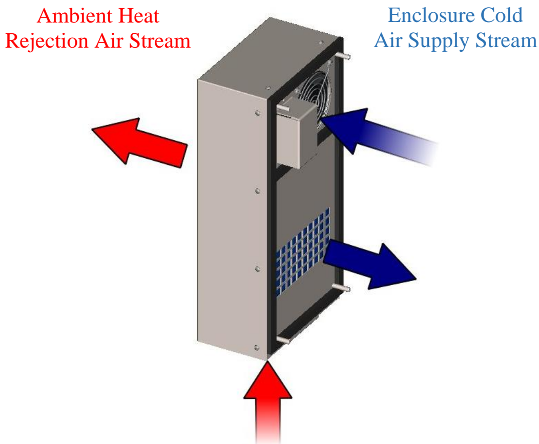
Figure 1: Air Flow
