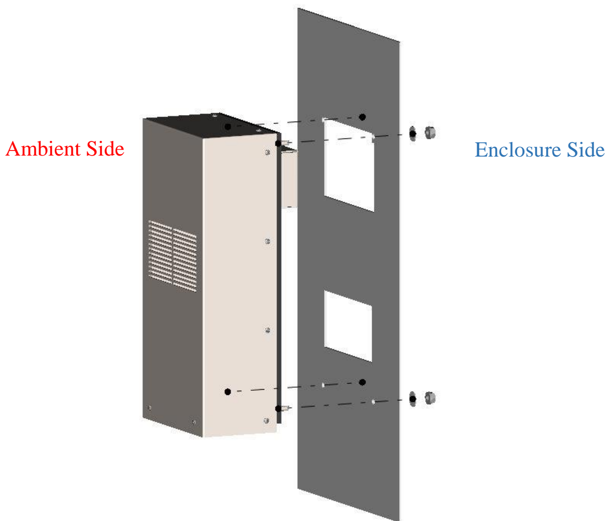
Figure 2: TMS Mounted
