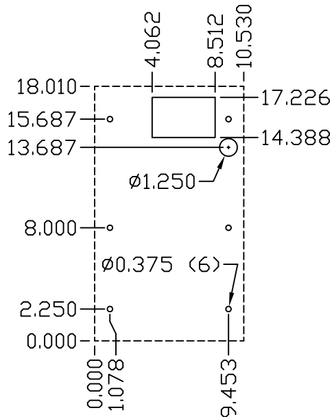
IQ300FPW INTAKE CUT OUT DRAWING
