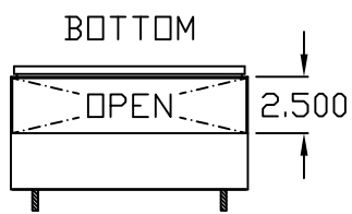
IQ300FPW INTAKE CUT OUT DRAWING
