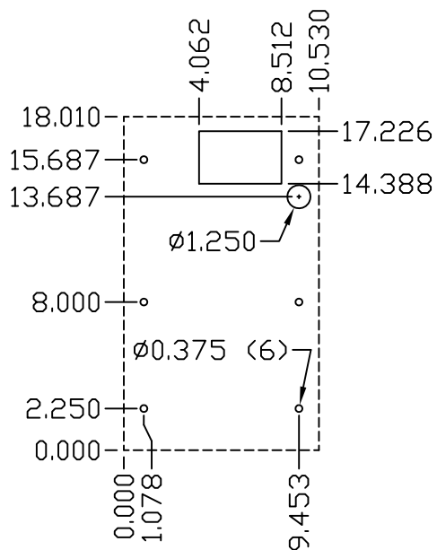
IQ300FPW EXHAUST CUT OUT DRAWING
